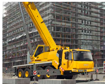
GMK4100L-1
